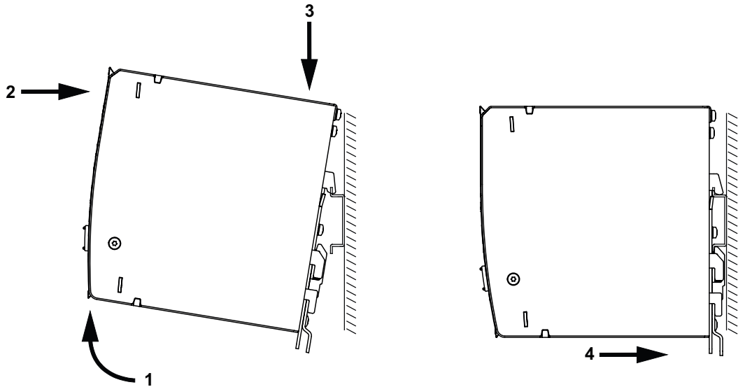
Figure 13: Mounting the Product on the DIN rail
