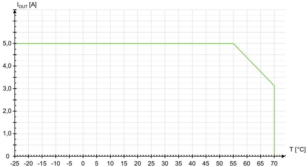
Figure 9: Derating (Temperature-Dependent)
