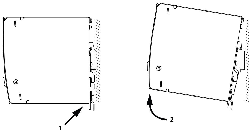
Figure 14: Removing the Product from the DIN Rail
