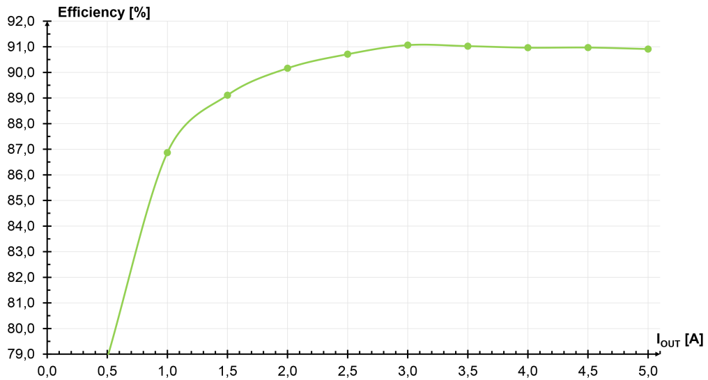
Figure 7: Efficiency at 230 VAC
