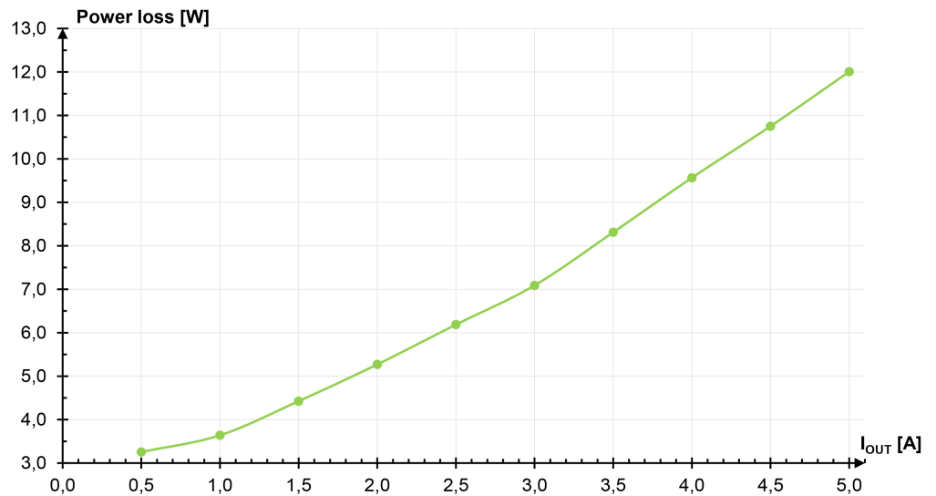
Figure 8: Power loss at 230 VAC
