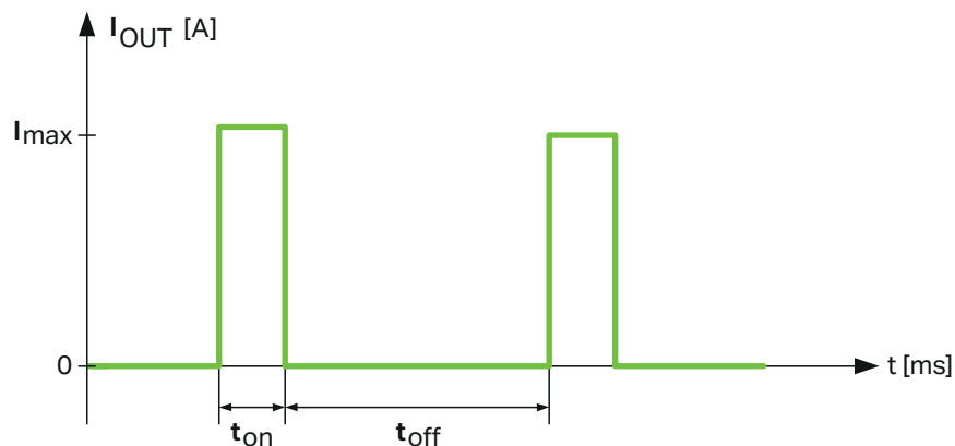
Figure 10: Hiccup-Mode
